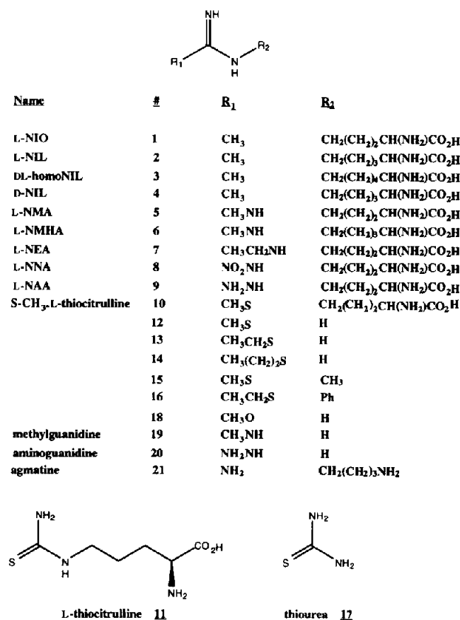
Figure 1. Structures of compounds 1–21.
